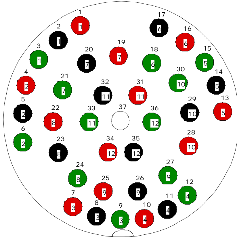
SBE Male Wiring Side
