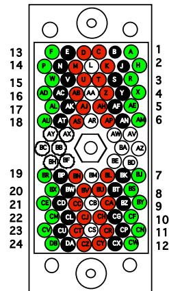
FEMALE WIRING SIDE (402)
